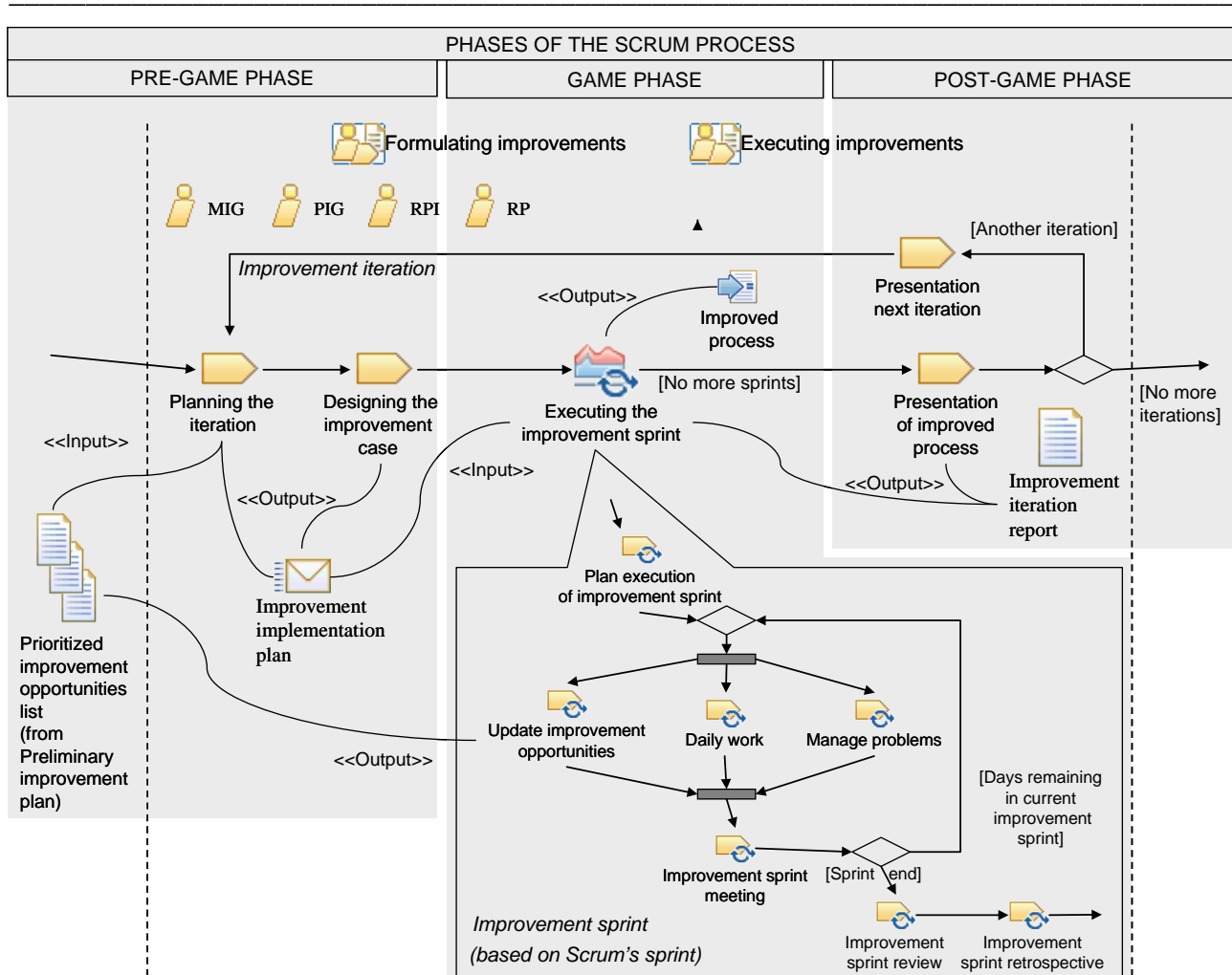
Figure 3. Diagram- activities of the Lightweight process to incorporate improvements
