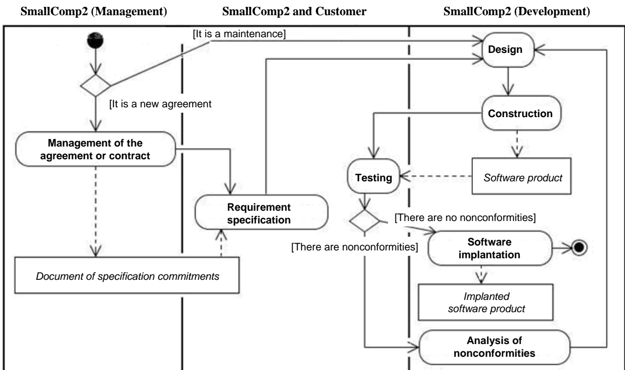
Figure 5. Activity diagram for SmallComp2
