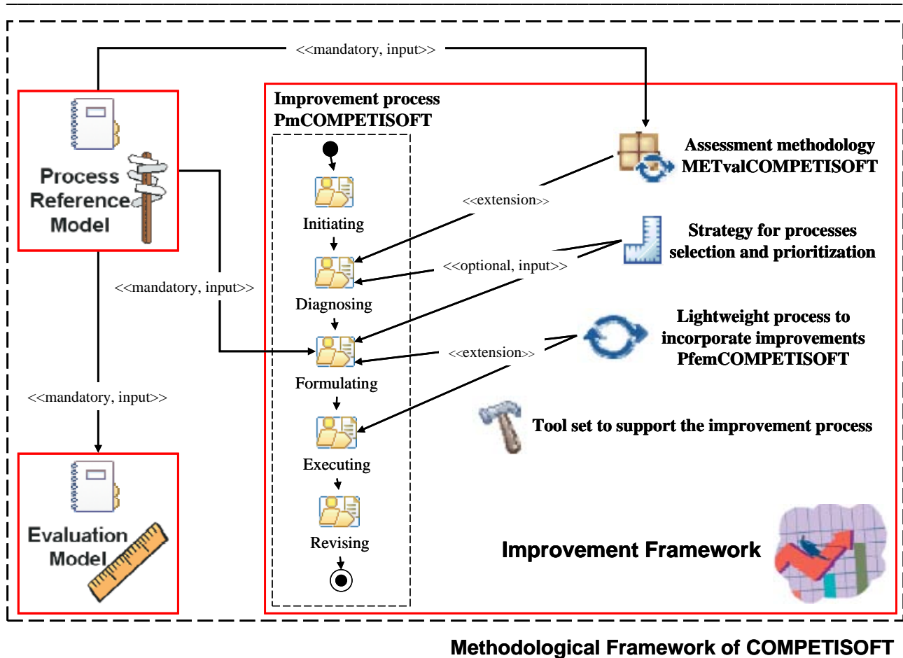
Figure 1. Overview of the Improvement framework and Methodological Framework of COMPETISOFT
