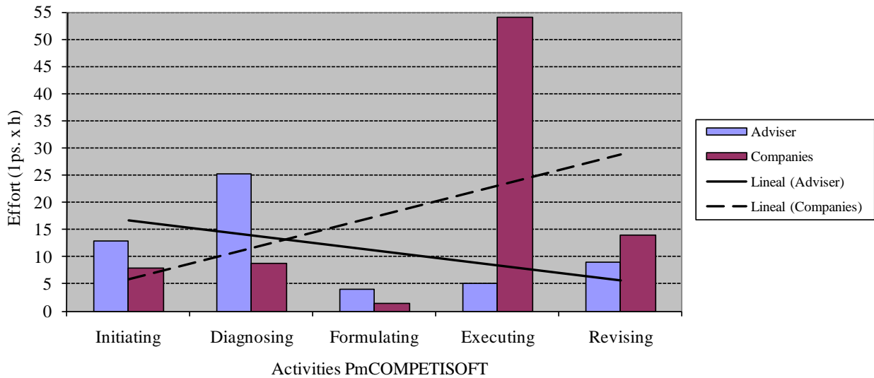
Figure 6. Distribution and tendency of effort in the case studies.
