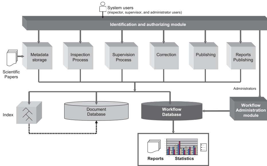
Figure 2: System architecture
