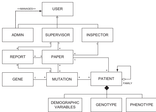
Figure 3: Data Model
