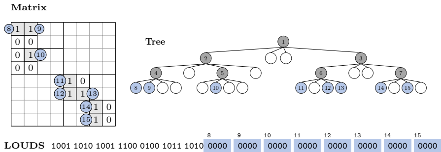
Fig. 1. An 8 \times 8 matrix (left, above), its corresponding k^2 -tree (right, above), and its cardinal LOUDS representation (below); the highlighted leaves 0000 are not represented.
