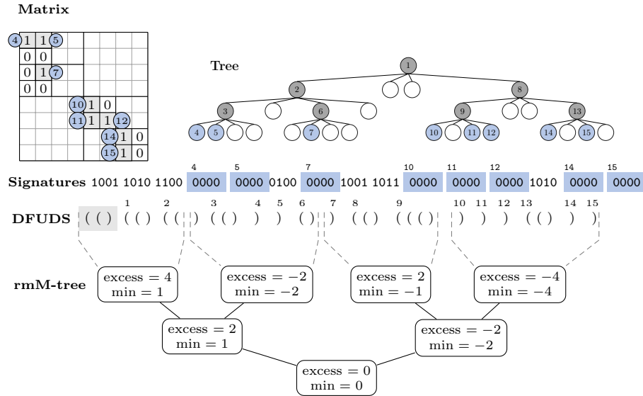
Fig. 2. Cardinal DFUDS representation of the same k^2 -tree of Fig. 1, using block size b = 8 for the rmM-tree.
